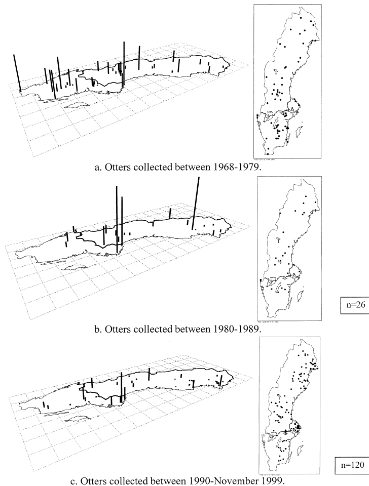
Fig. 2a–c. The left column: concentrations of total PCB in the otters (traumatically killed) that has been analysed. The right column: sampling localities of all otters found dead during three decades.
